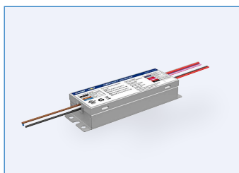
R83006 RENO-EM-E08 Emergency LED Driver (100-347V AC, 50-60Hz, 8W)
