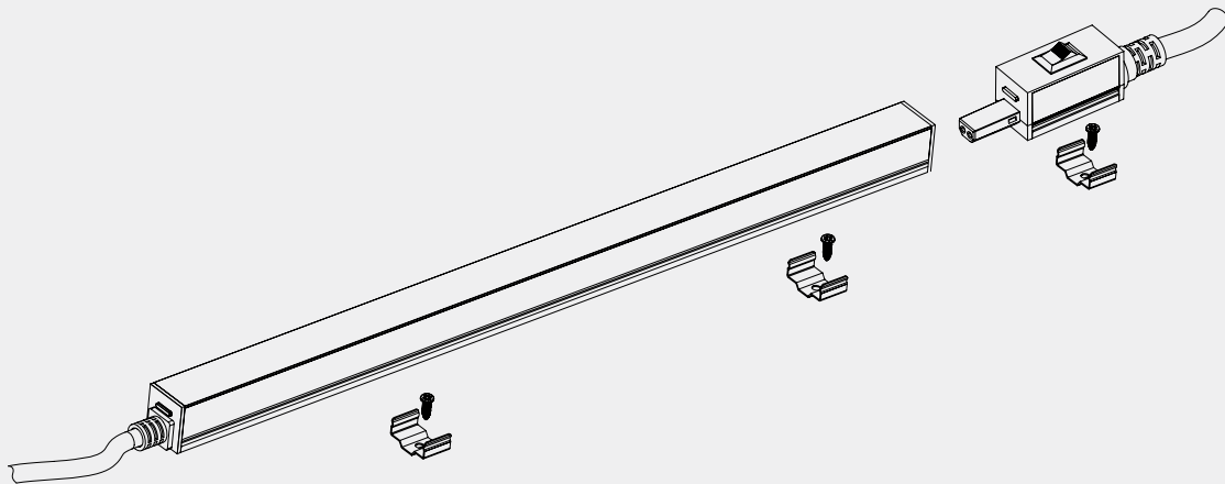
Assembly Overview (with inline On/Off Switch)
