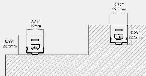
Surface Mounting | Recessed Mounting
