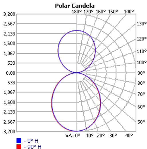
LUMINOUS INTENSITY DISTRIBUTION
